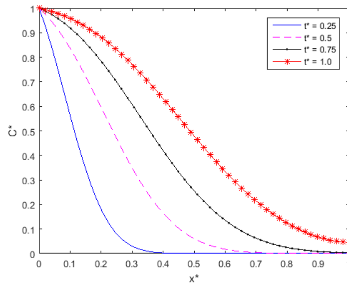
Fig. 3. One-dimensional profile c^*(x^*) at t^* = 0.25, 0.50, 0.75, 1.0 for Pe \gg 1 (advection-dominated; concentration persists downstream).
