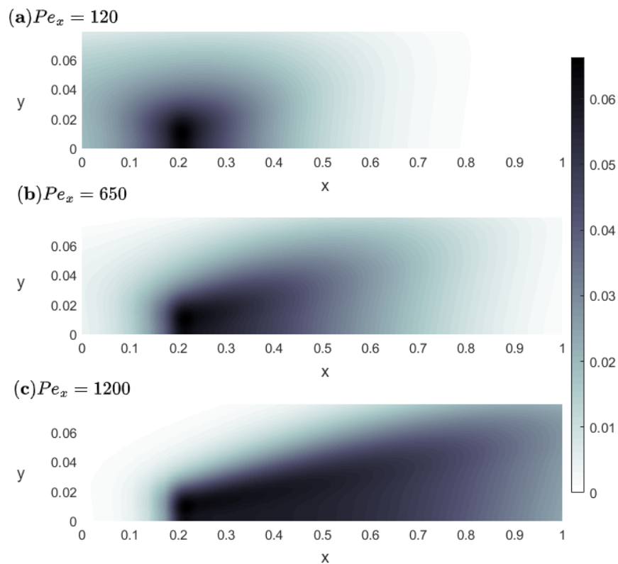
Fig. 7. Two-dimensional concentration distribution at t = 0.35 for (a) Pe_x = 120 , (b) Pe_x = 650 , (c) Pe_x = 1200 . Higher Pe elongates the plume downstream.
