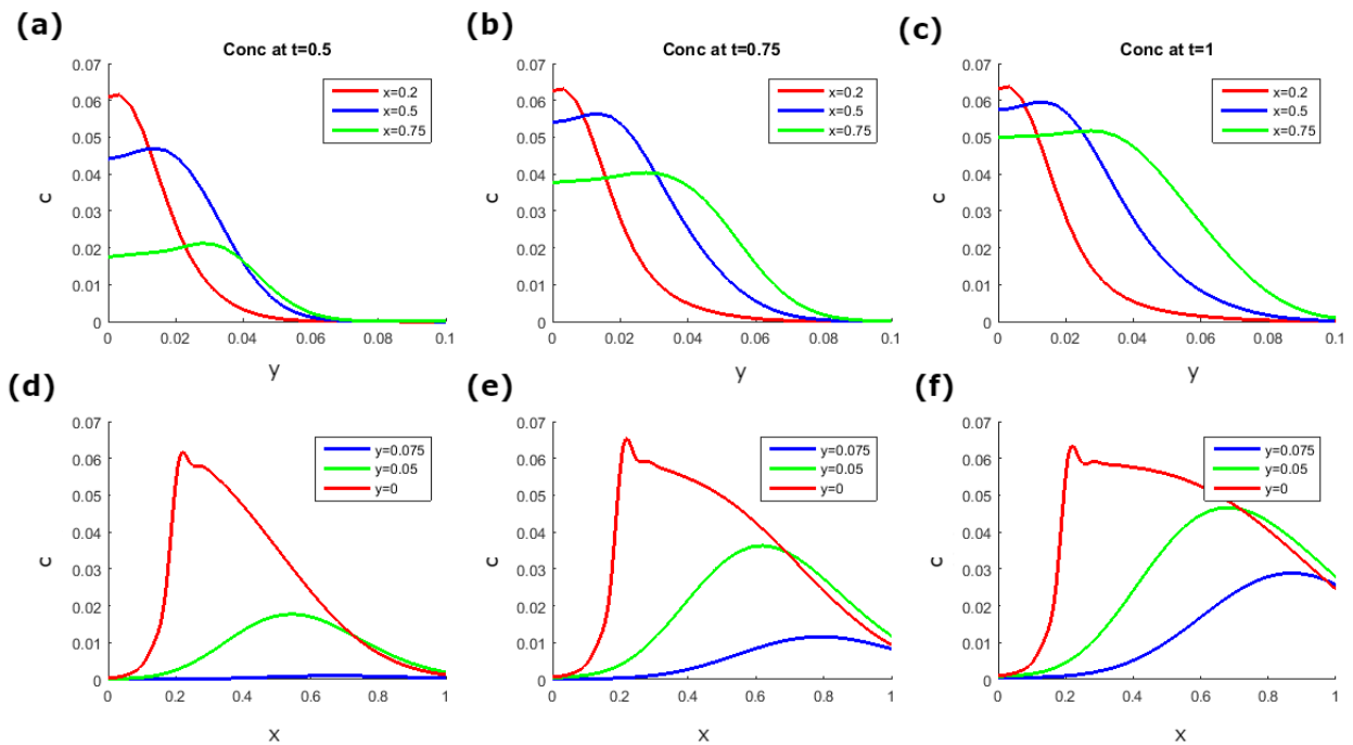
Fig. 6. Concentration profiles at different positions and times: (a)–(c) across the width at t = 0.5, 0.75, 1 ; (d)–(f) along the channel for y = 0, 0.05, 0.075 .
