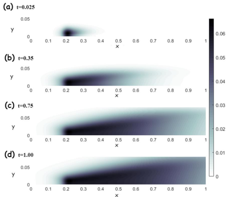
Fig. 4. Concentration attenuation of an instantaneous point source at (0.2, 0.005) for (a) t = 0.025 , (b) 0.35, (c) 0.75, (d) 1.00; the patch expands and translates downstream.
