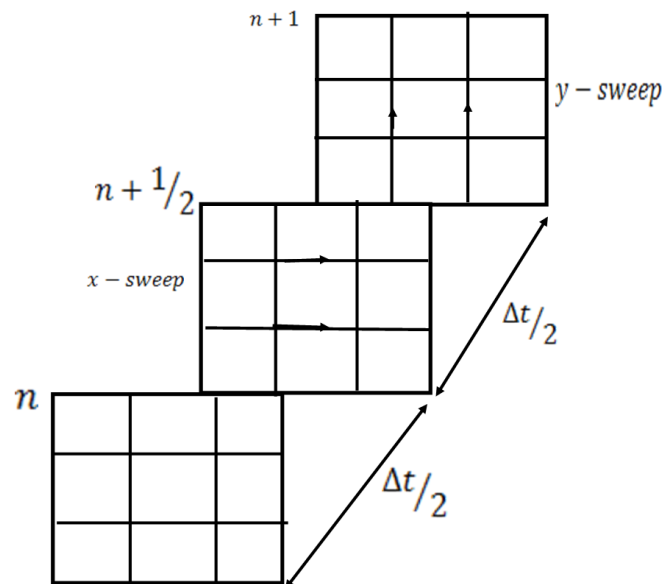
Fig. 1. Illustration of the grid system for the ADI method: the x-sweep (implicit in x at n + 1/2 ) followed by the y-sweep (implicit in y at n + 1 ).
